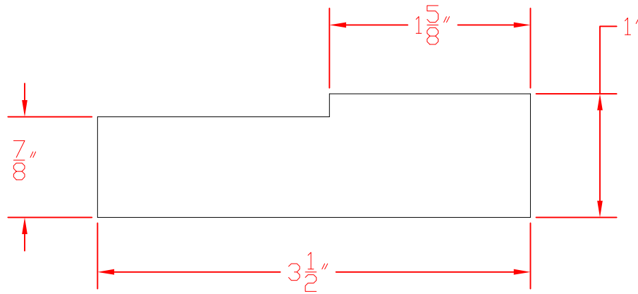
4" STANDARD SURROUND
