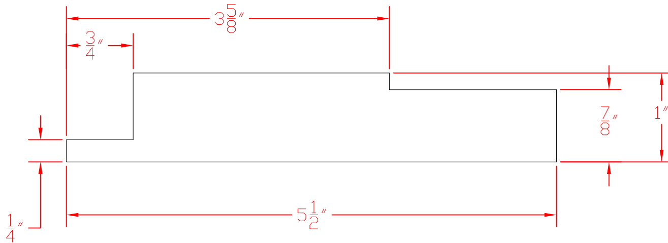
6" J-POCKET SURROUND
