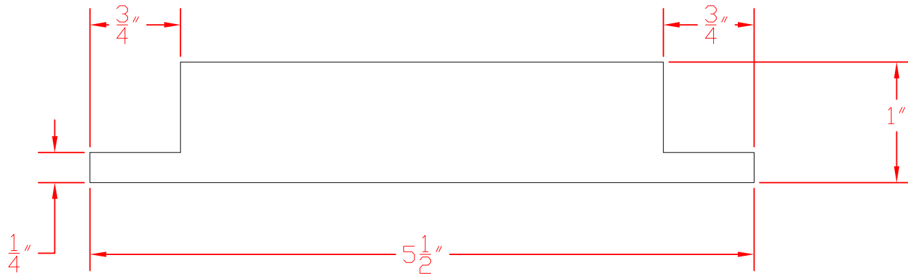
6" DOUBLE J-POCKET
